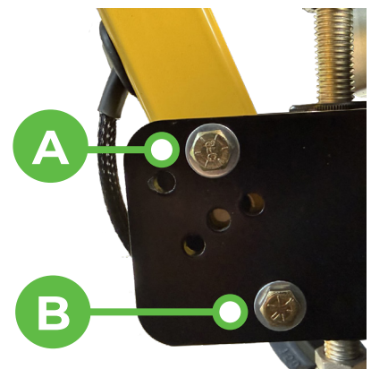
A. Height/angle adjustment bolt B. Frame attachment bolt
